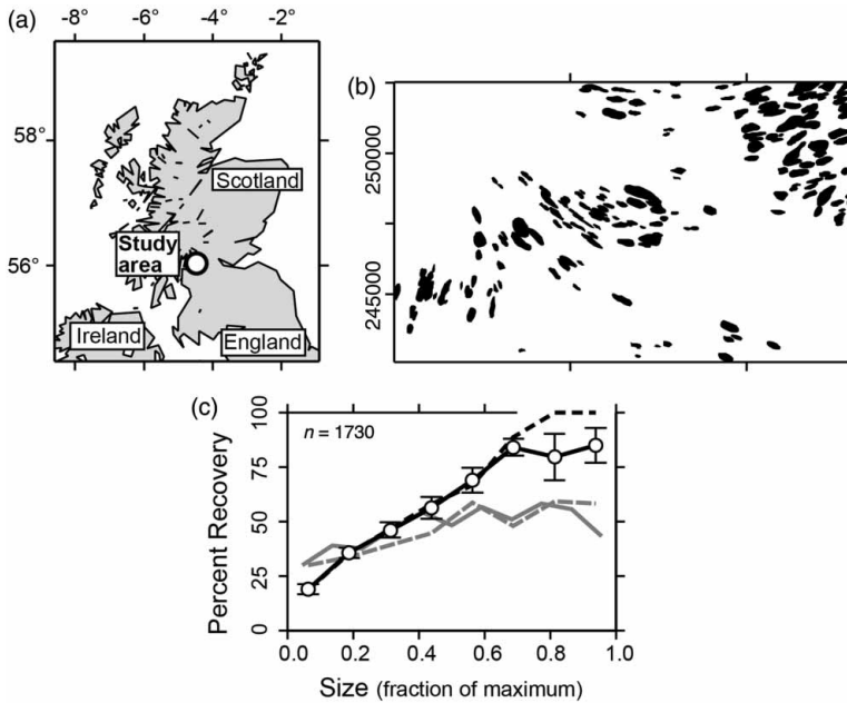
Figure 1. (a) Location of the study area. (b) Drumlins (black) in the area as mapped by Smith et al. (2006). (c) Recovery (i.e. ‘completeness’) as a function of size; synthesis of a manual mapping pilot study for which the methodology was as here (see ‘Interpretive Mapping’) but applied to 10 DEMs equivalent to Maps 1–5 using only one mapper (Arumgam). Black line is for height, H , and grey lines are for width W (solid) and length L (dashed). Circles are means with their standard errors for the 10 DEMs, and dashed line is for medians. H , W , and L have bin widths of 2.5, 25 and 100 m, respectively. At the upper end, bins with two or fewer input data are omitted, giving maxima of 20, 275 and 800 m, respectively. All data are plotted centrally within bins.
