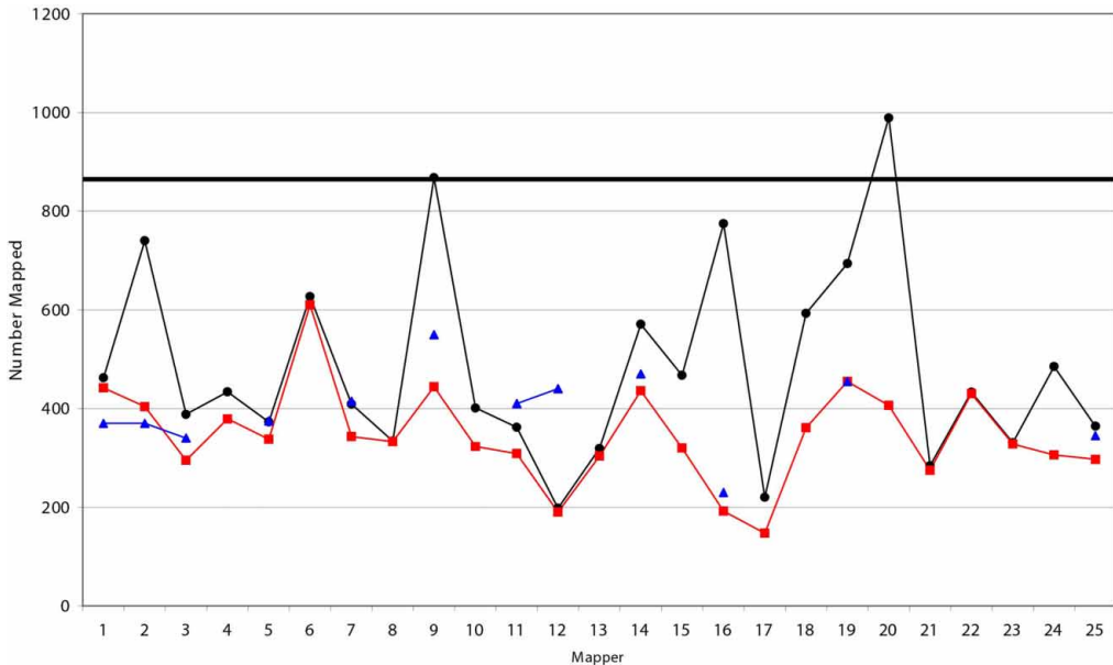
Figure 2. Number of drumlins mapped per individual interpreter (black circles) and the number correct (red squares). Blue triangles are for the number correctly mapped in synthetic DEMs with parallel conformity, scaled ( \times 5 ) to allow comparison. Horizontal black line is the number of drumlins in the synthetics. This was known to the mappers.
